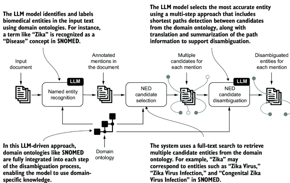
Figure 8.2 Workflow for a NED system designed to use LLMs and domain-specific ontologies, such as SNOMED, for biomedical text processing. Each stage of this workflow involves interactions to accurately disambiguate entities in the input text.
