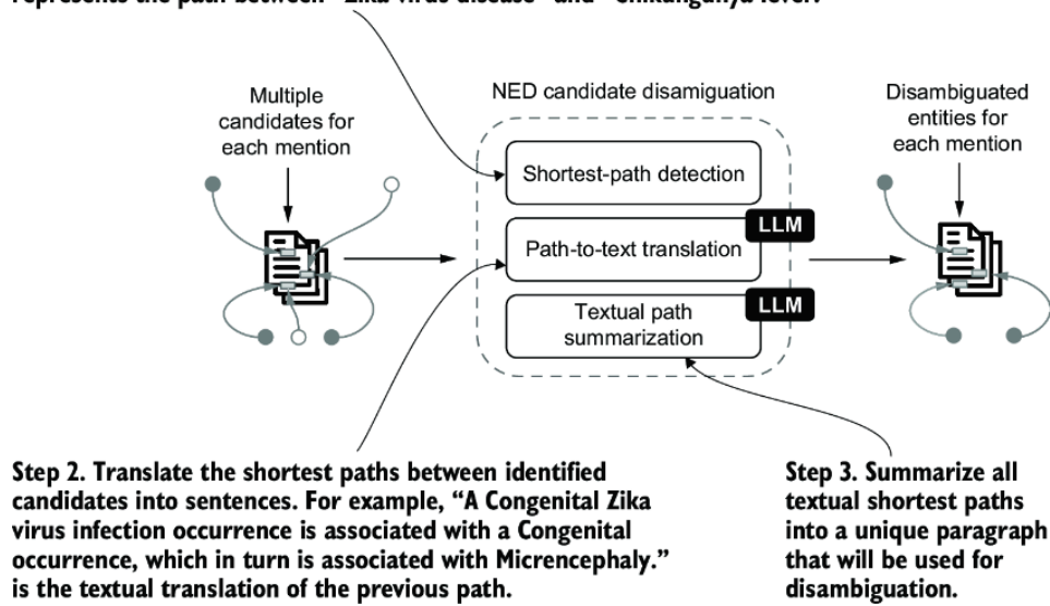
Figure 8.6 NED CD steps: (1) detecting the shortest paths between all the candidates related to the entity mentions in the sentence; (2) translating detected paths into natural language sentences; (3) summarizing those sentences into useful text for disambiguation
