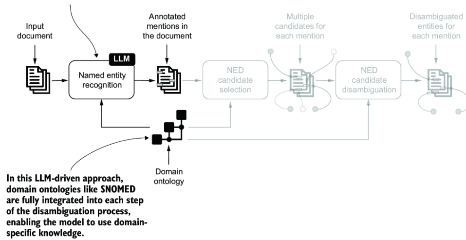
Figure 8.3 The first stage of NED is NER. In our scenario, named entities are derived directly from the ontology. In SNOMED, categories are defined by the ontology’s first-level nodes, whose information is propagated to all the other nodes.
