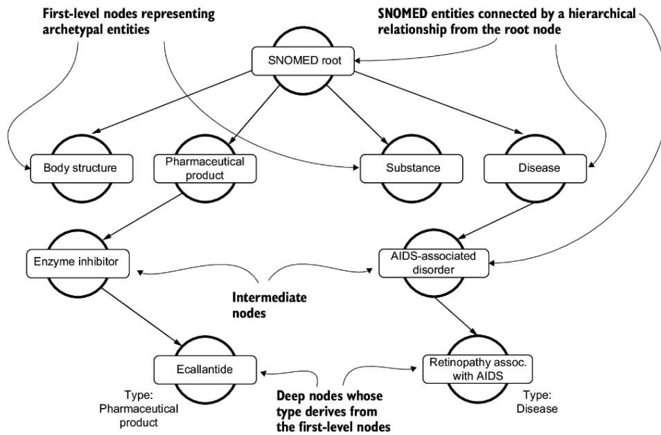
Figure 8.1 A sample of SNOMED's hierarchical structure. Nodes on deeper levels can be categorized using information from first-level nodes, which are the ontology's archetypal entities.
